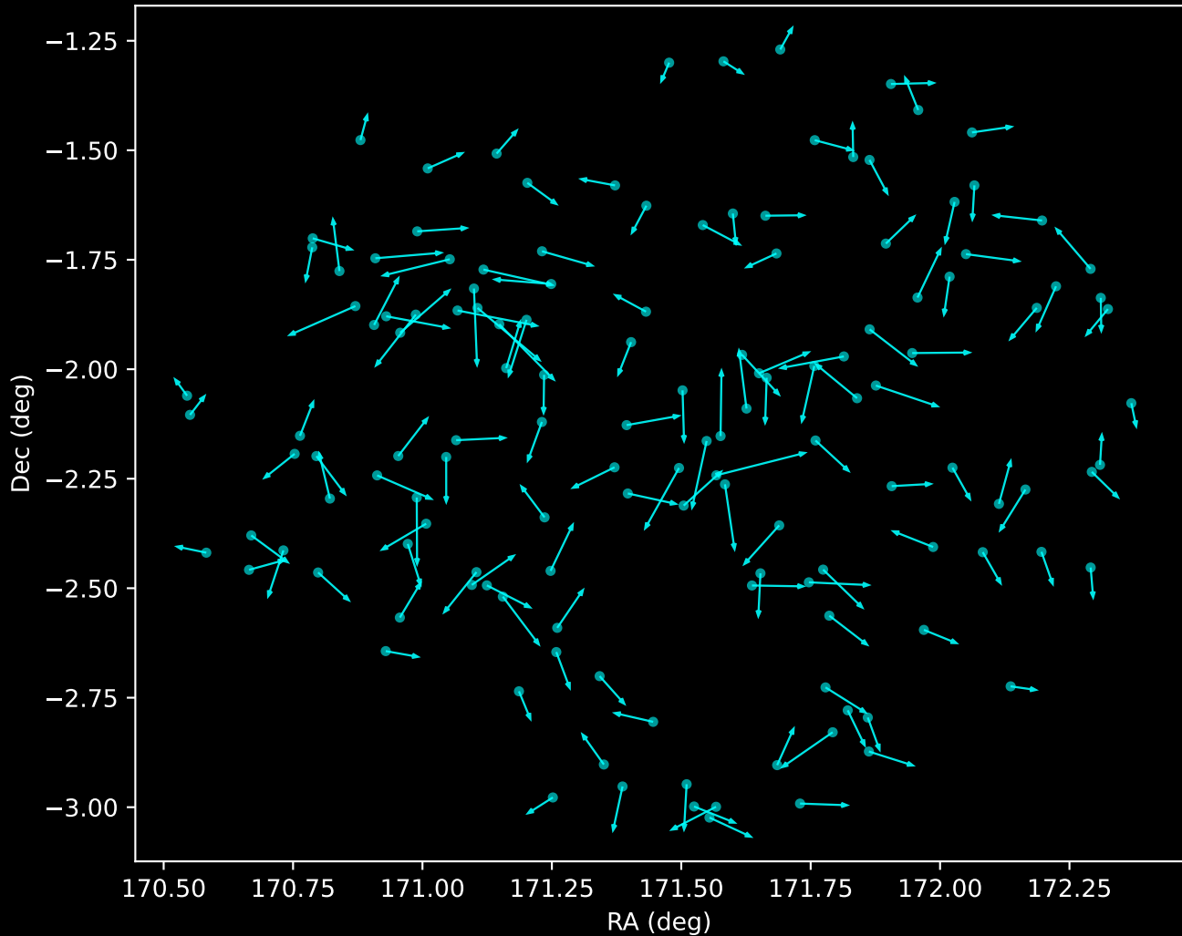
GALAH DR4 Noise Stream Proper Motion Vectors (n=140)
