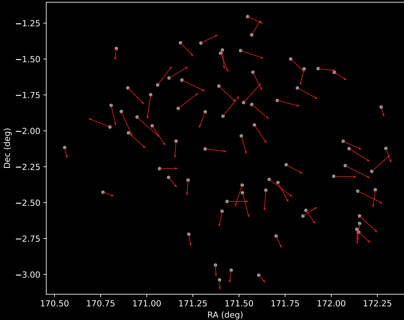
GALAH DR4 Cluster 6 Proper Motion Vectors (n=70)
