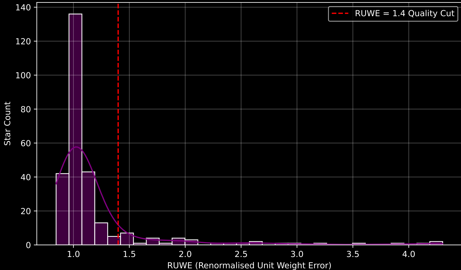
GALAH DR4 Field [1096] RUWE Distribution (n= 272)
