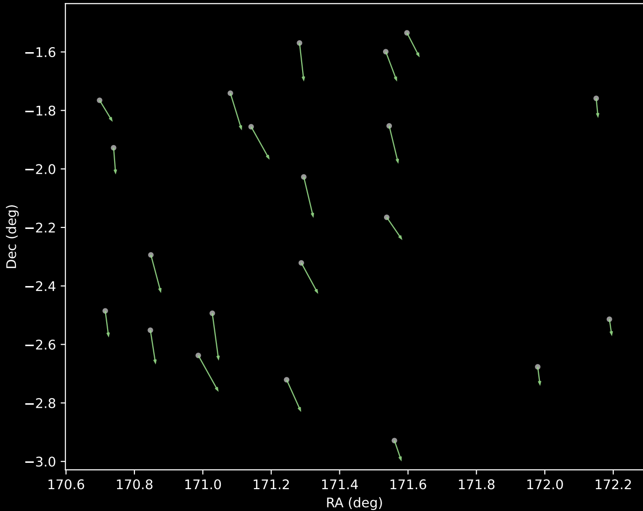
GALAH DR4 Cluster 5 Proper Motion Vectors (n=21)
