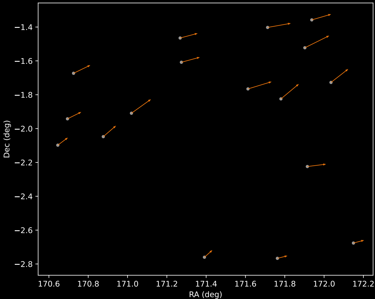
GALAH DR4 Cluster 2 Proper Motion Vectors (n=17)
