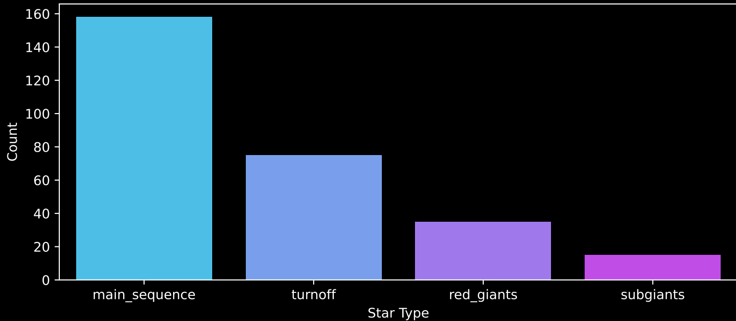
GALAH DR4 Field: [1096] Count plot of Star Type
